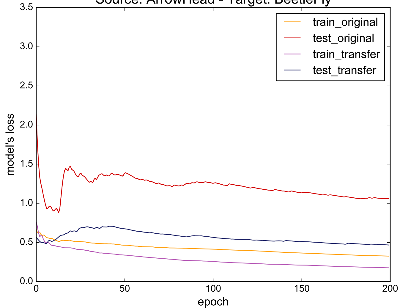
Source: ArrowHead - Target: BeetleFly
