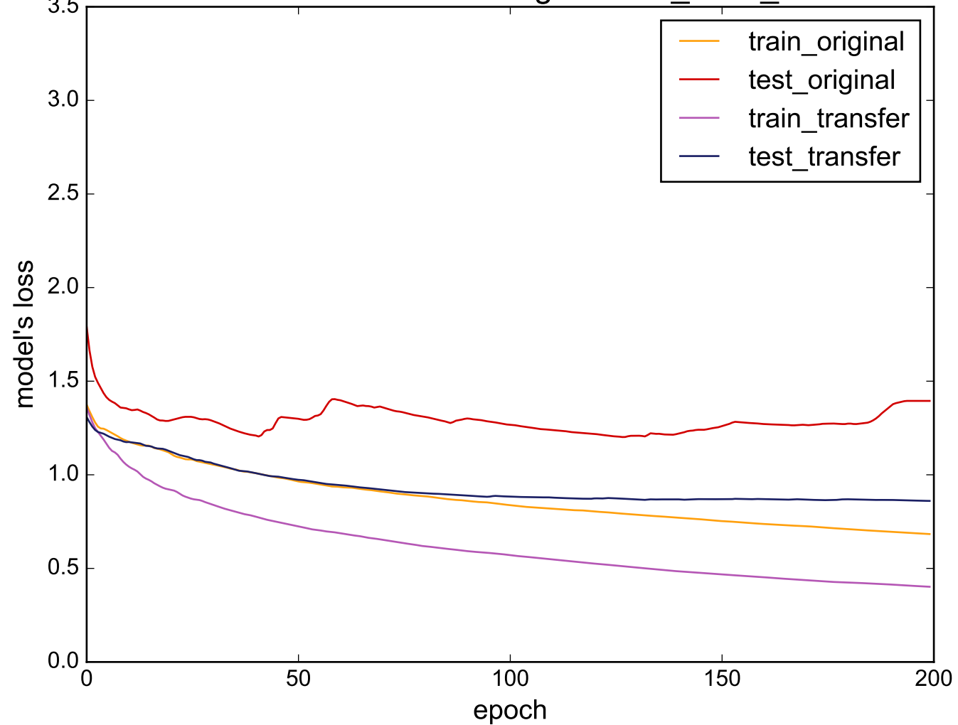
Source: ArrowHead - Target: CinC_ECG_torso
