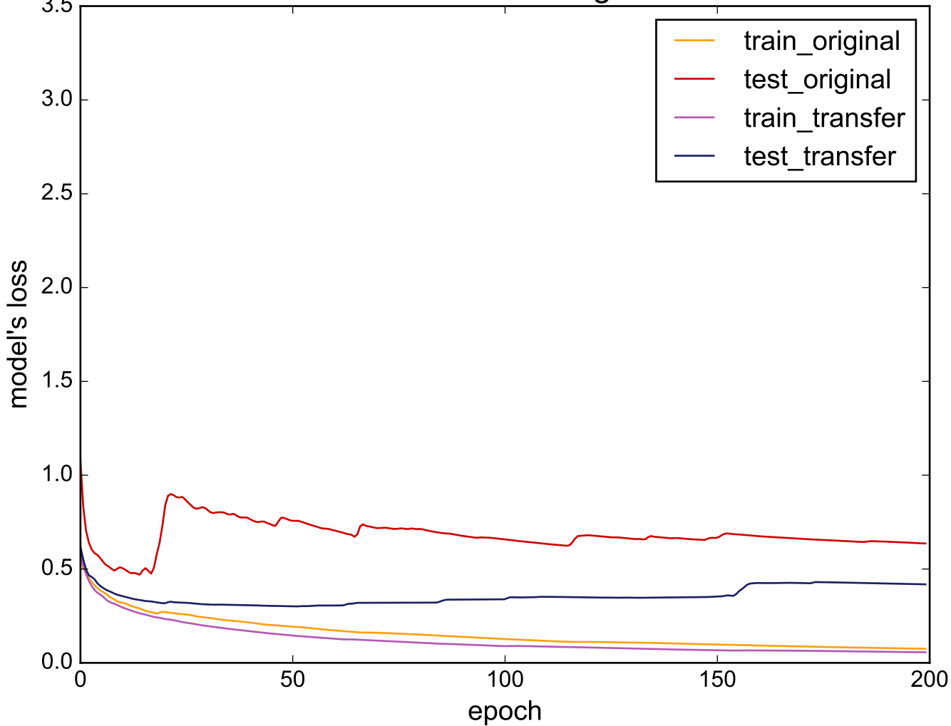
Source: ArrowHead - Target: ECG200
