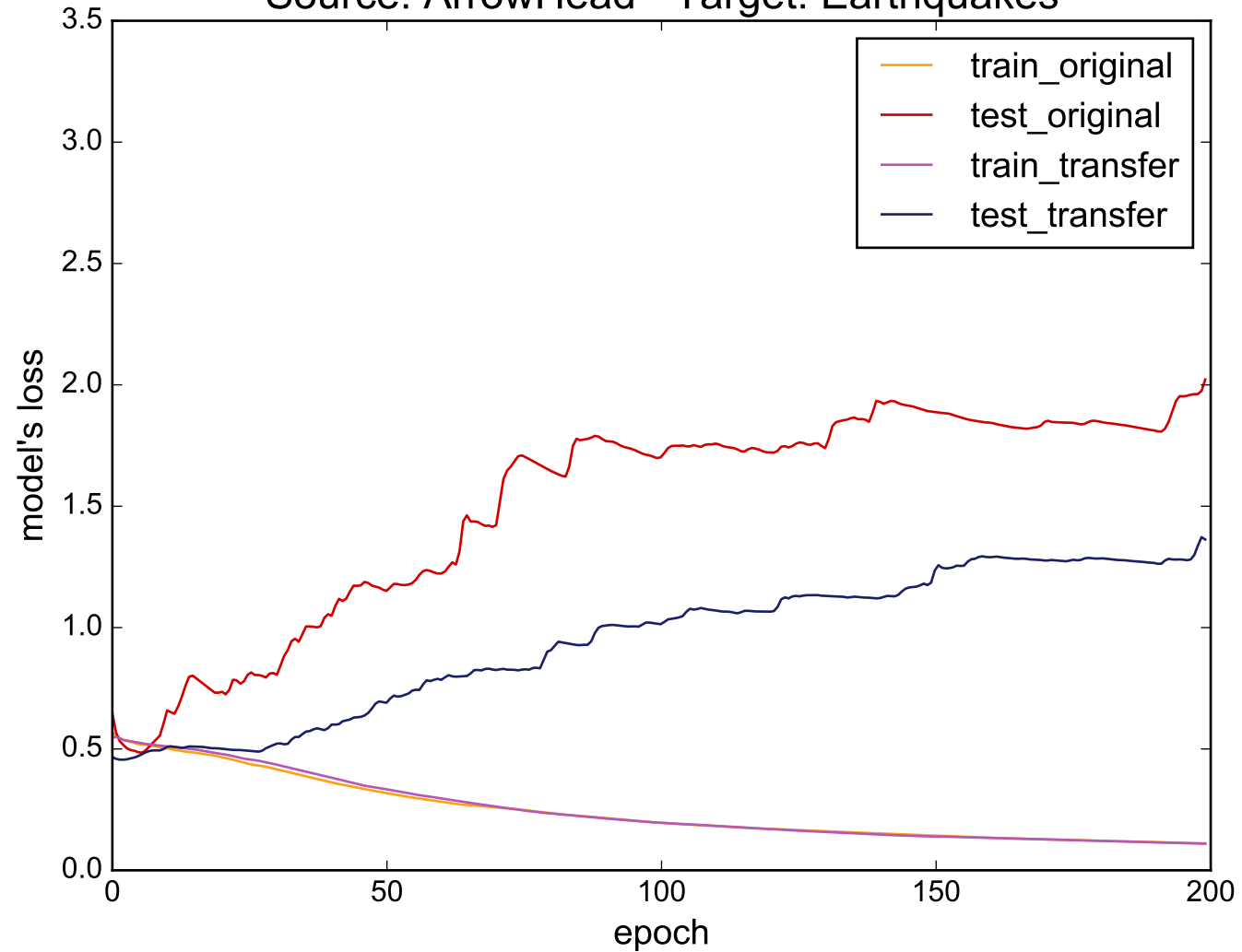
Source: ArrowHead - Target: Earthquakes
