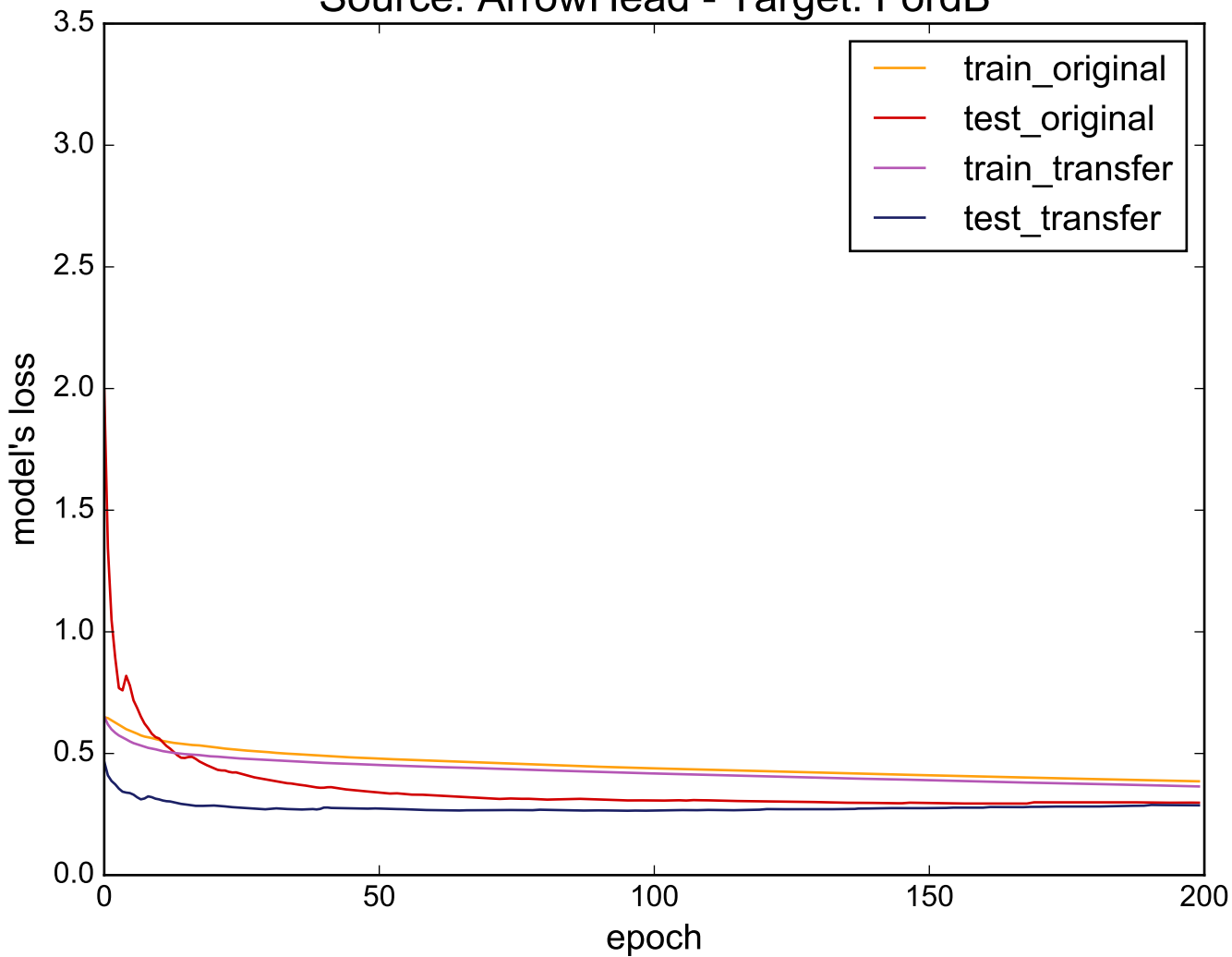
Source: ArrowHead - Target: FordB
