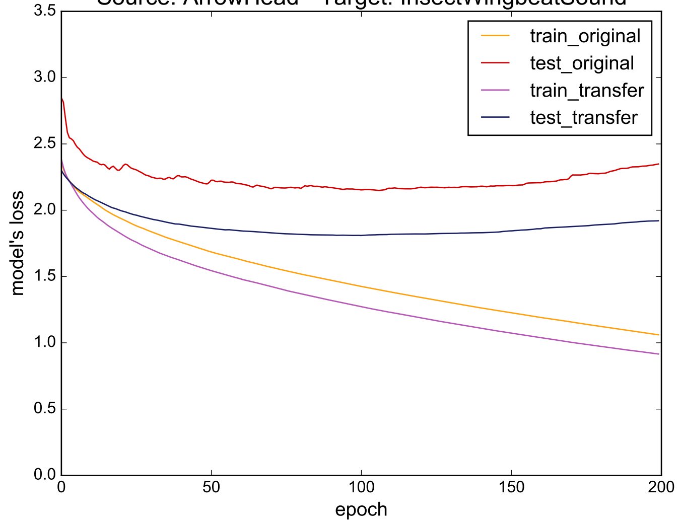
Source: ArrowHead - Target: InsectWingbeatSound
