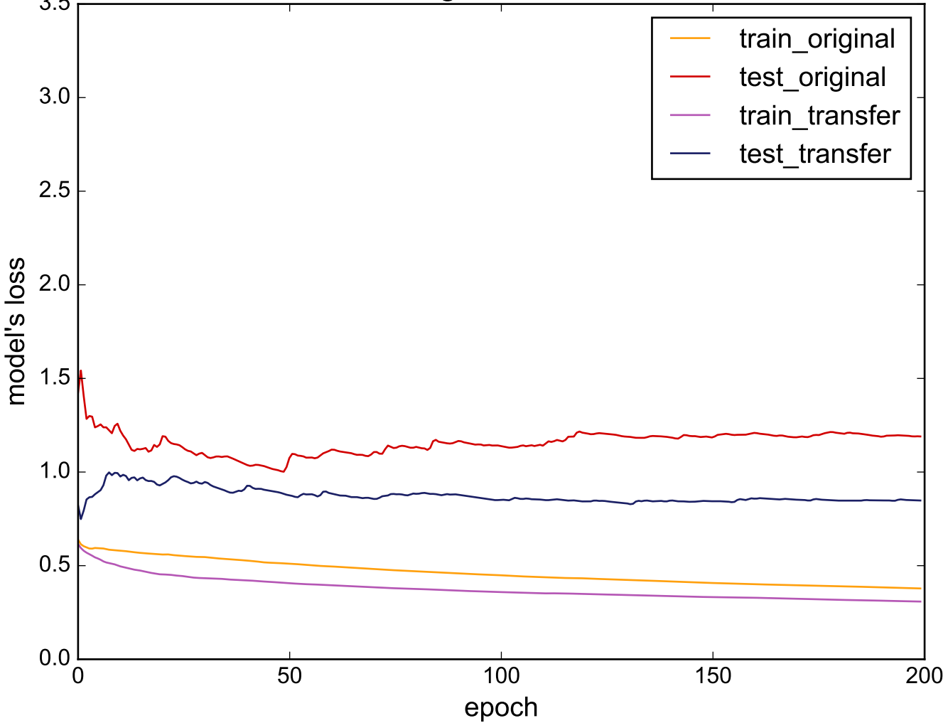
Source: ArrowHead - Target: MiddlePhalanxOutlineCorrect
