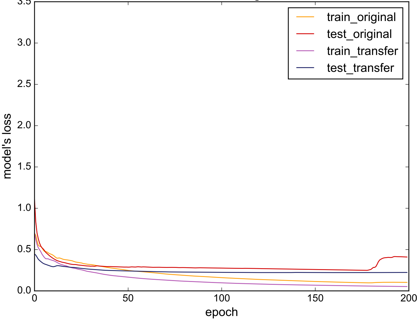
Source: ArrowHead - Target: MoteStrain
