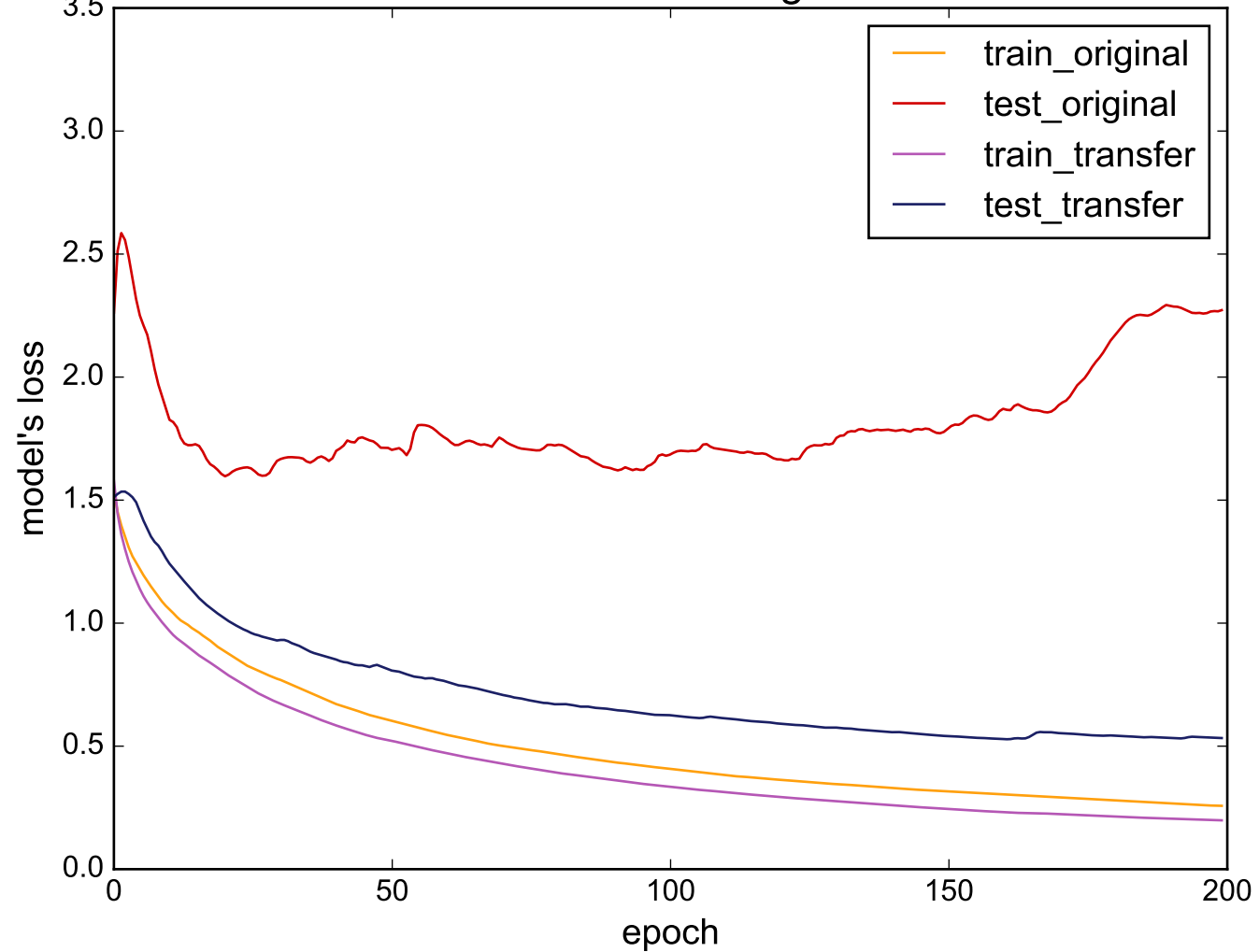
Source: ArrowHead - Target: OSULeaf
