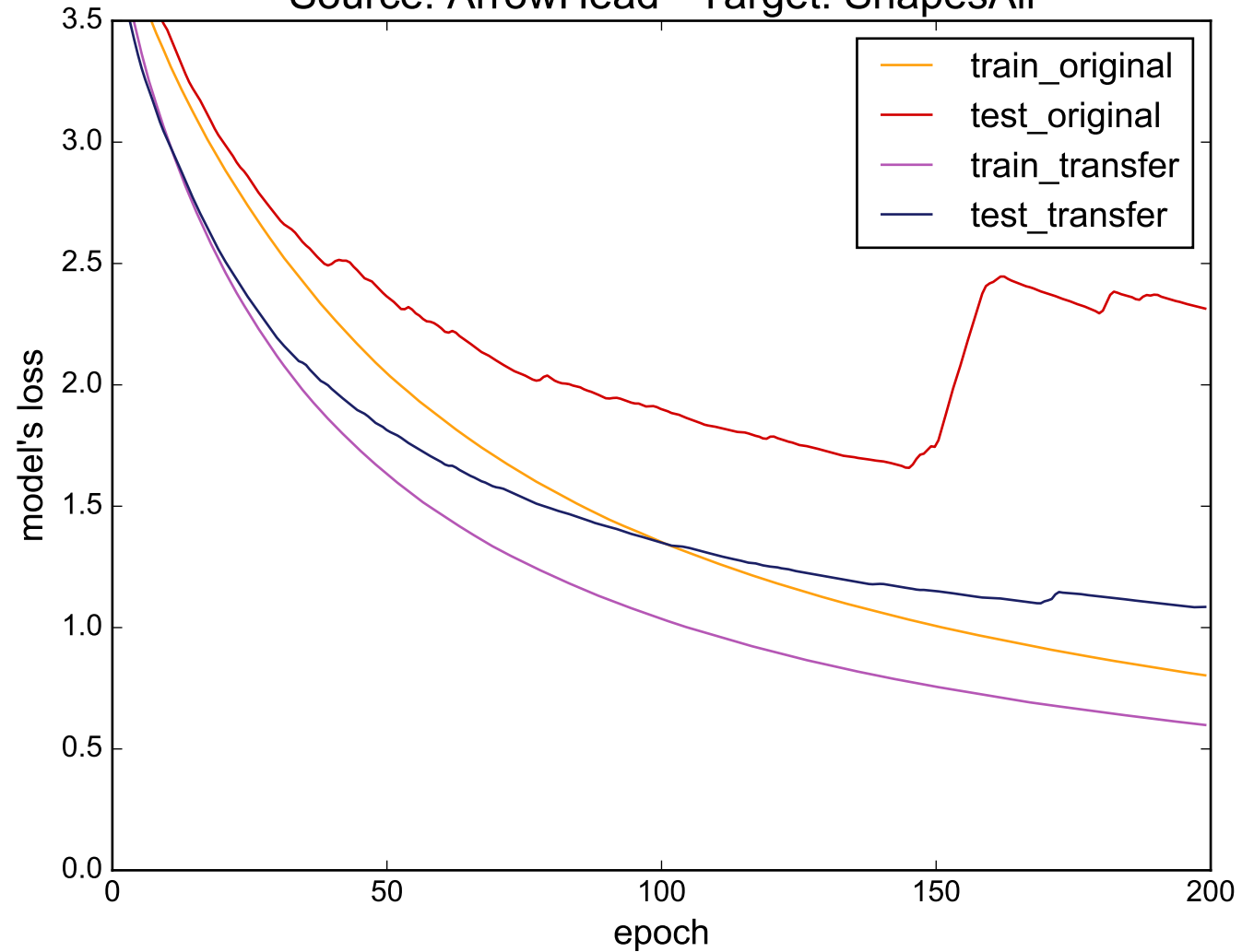
Source: ArrowHead - Target: ShapesAll
