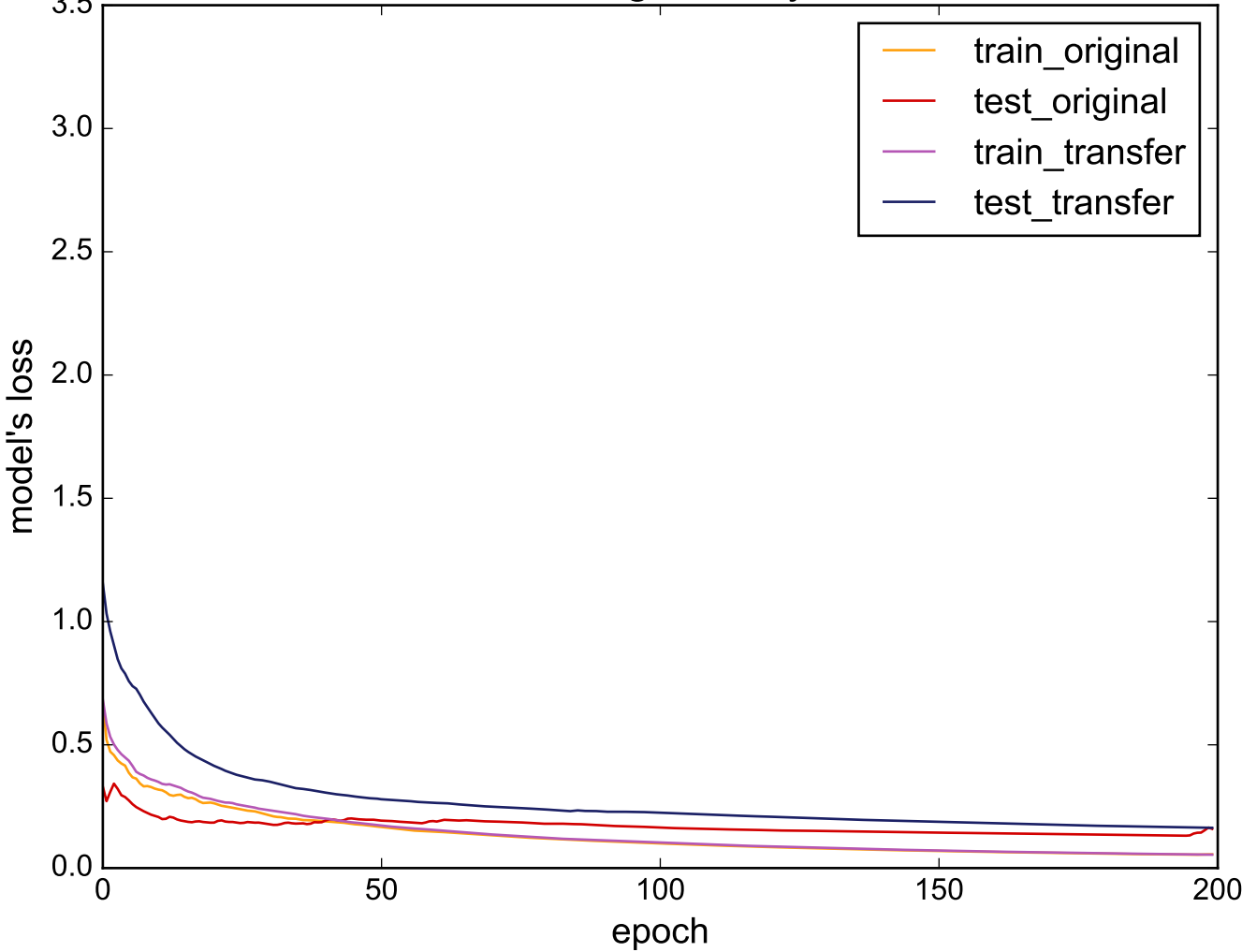
Source: ArrowHead - Target: SonyAIBORobotSurface
