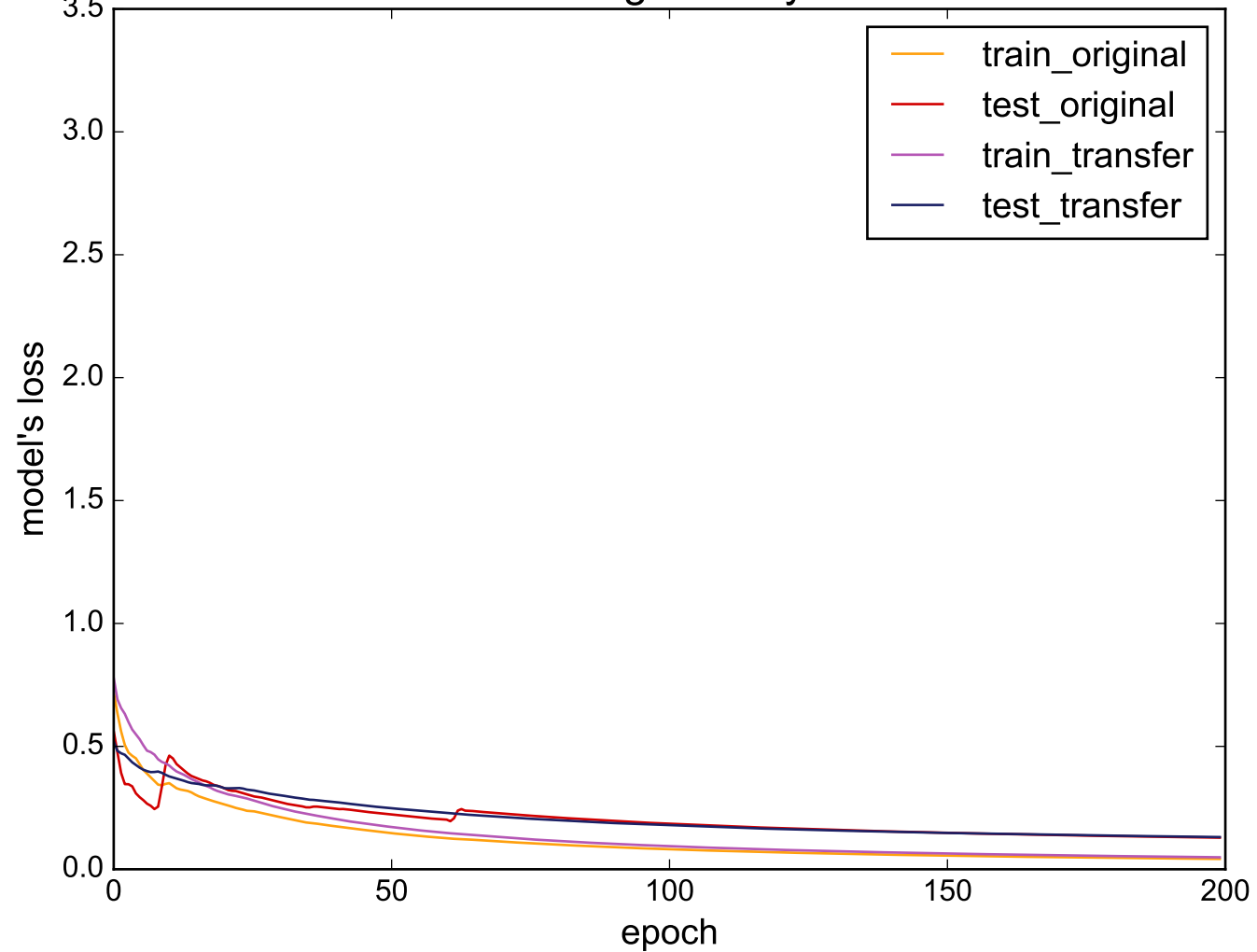
Source: ArrowHead - Target: SonyAIBORobotSurfaceII
