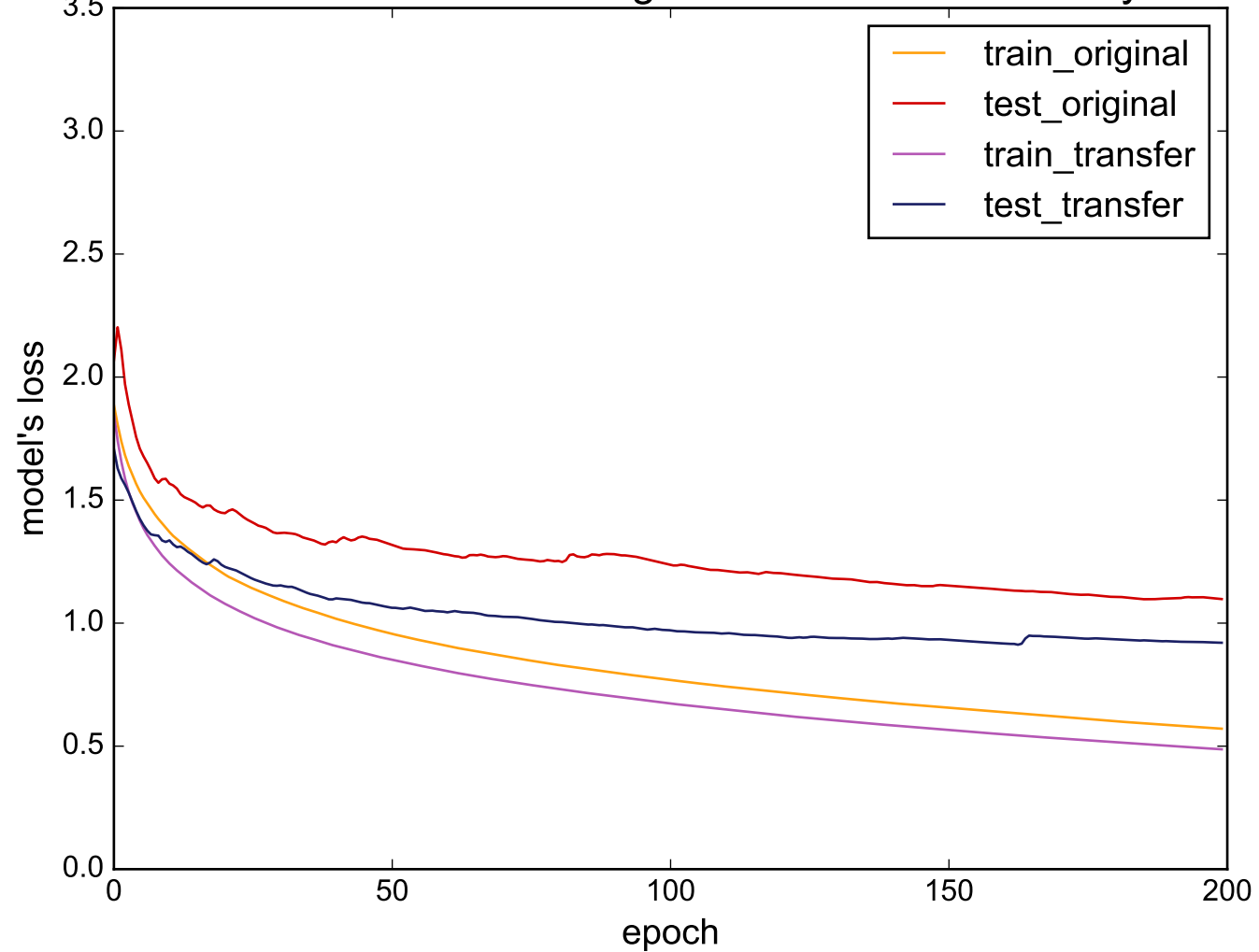
Source: ArrowHead - Target: UWaveGestureLibraryAll
