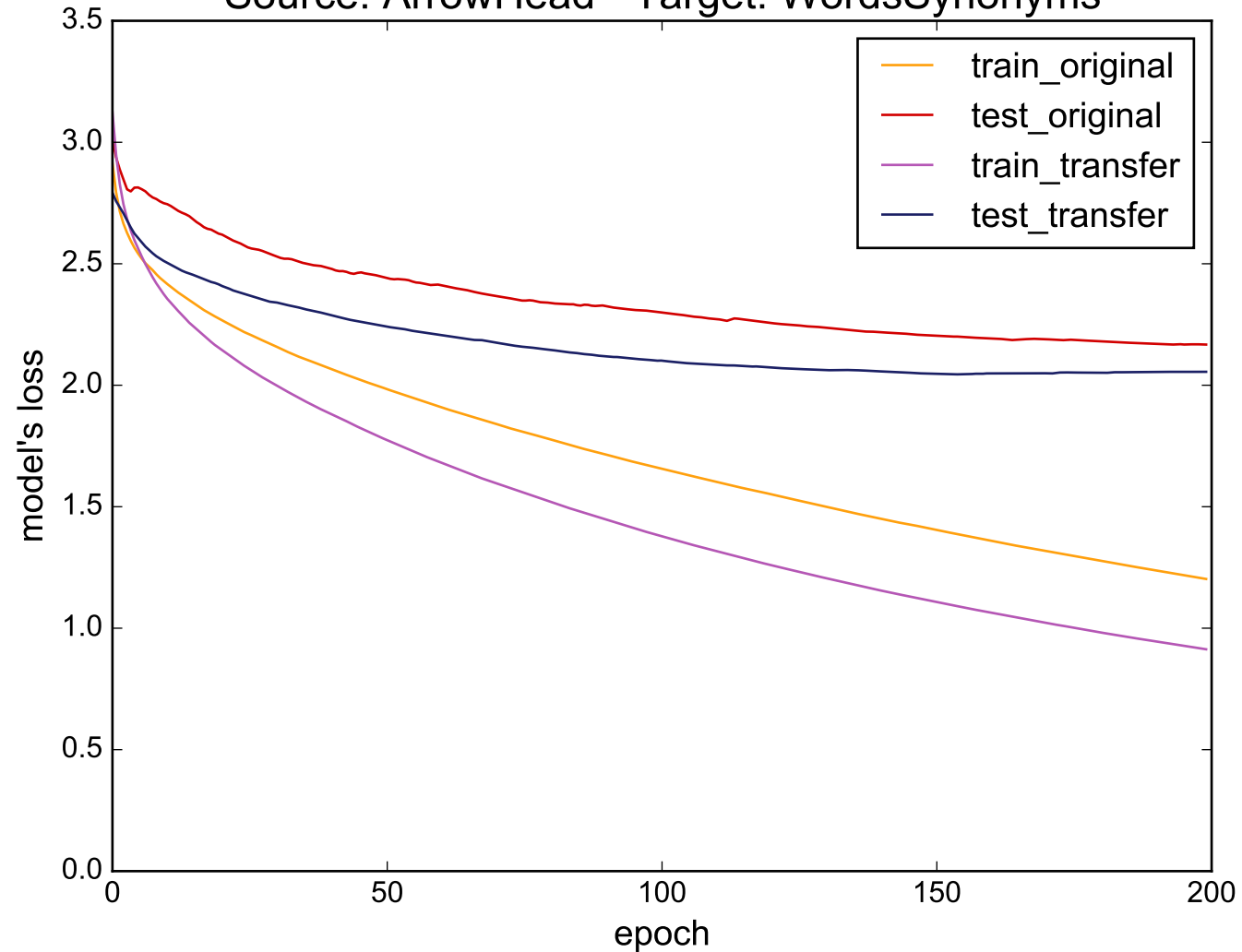
Source: ArrowHead - Target: WordsSynonyms
