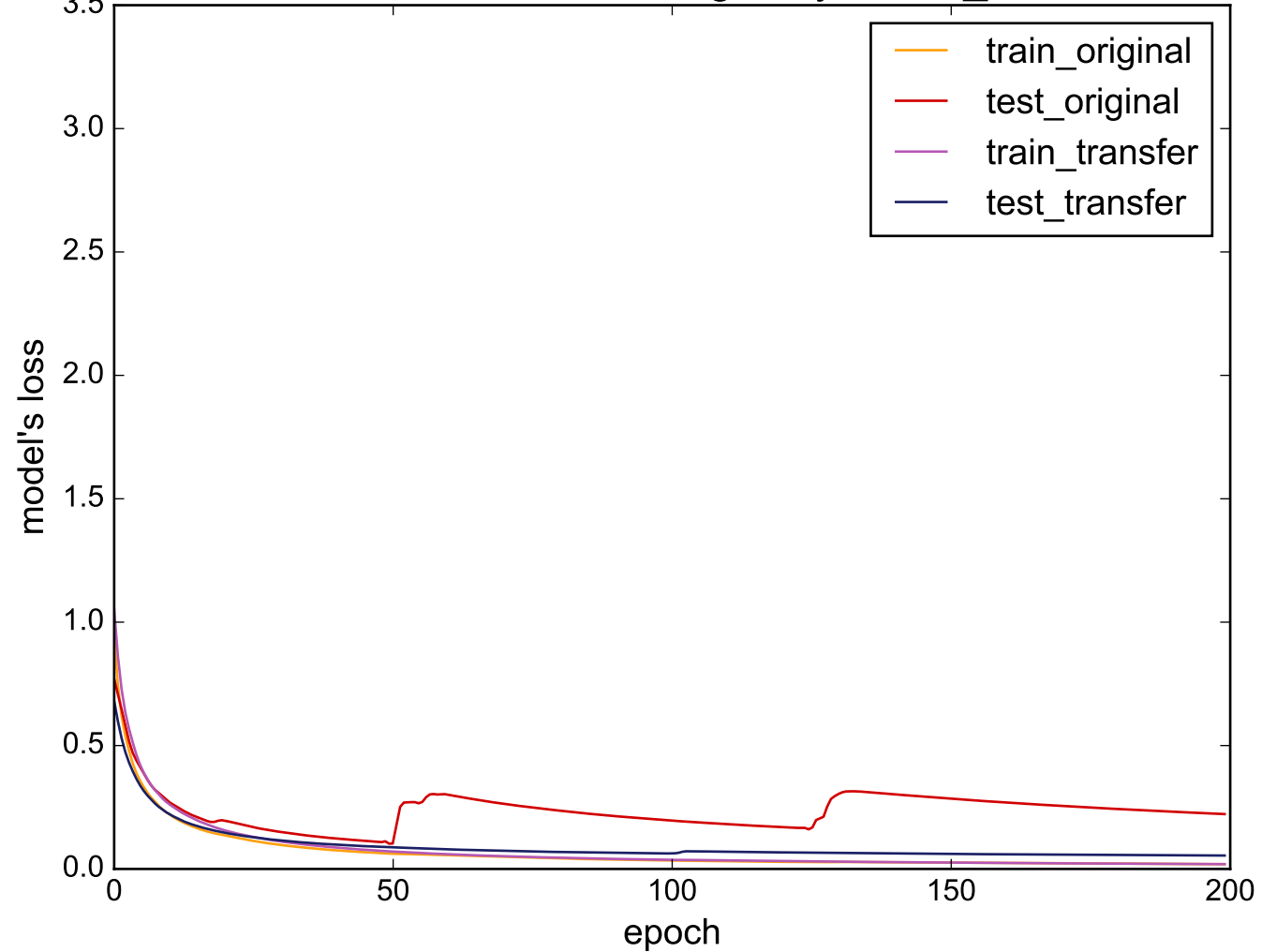
Source: ArrowHead - Target: synthetic_control
