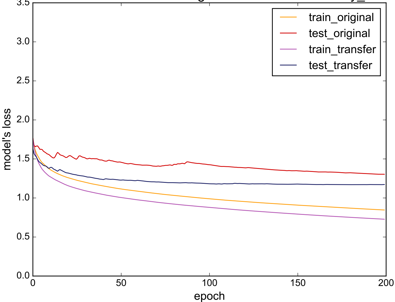
Source: ArrowHead - Target: uWaveGestureLibrary_Y
