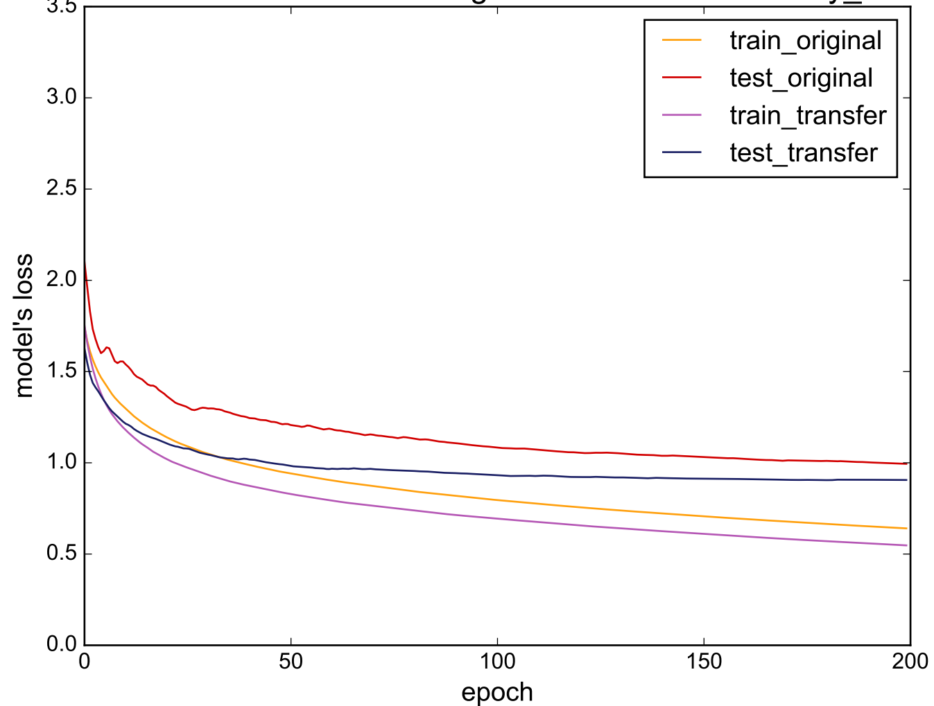
Source: ArrowHead - Target: uWaveGestureLibrary_Z
