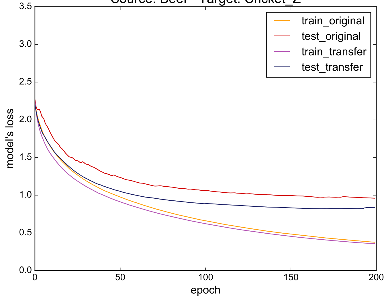
Source: Beef - Target: Cricket_Z
