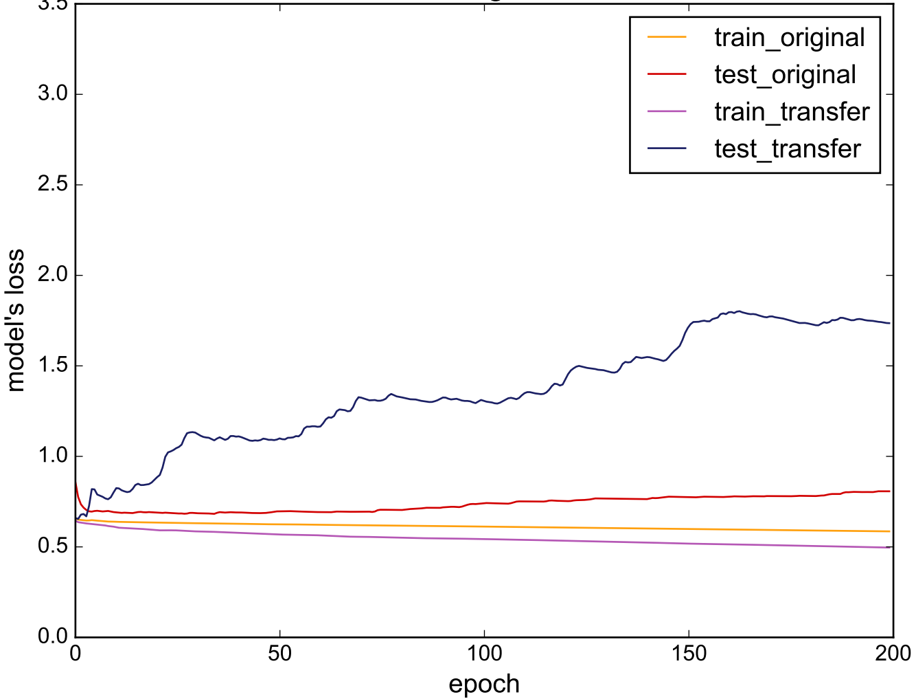
Source: Beef - Target: HandOutlines
