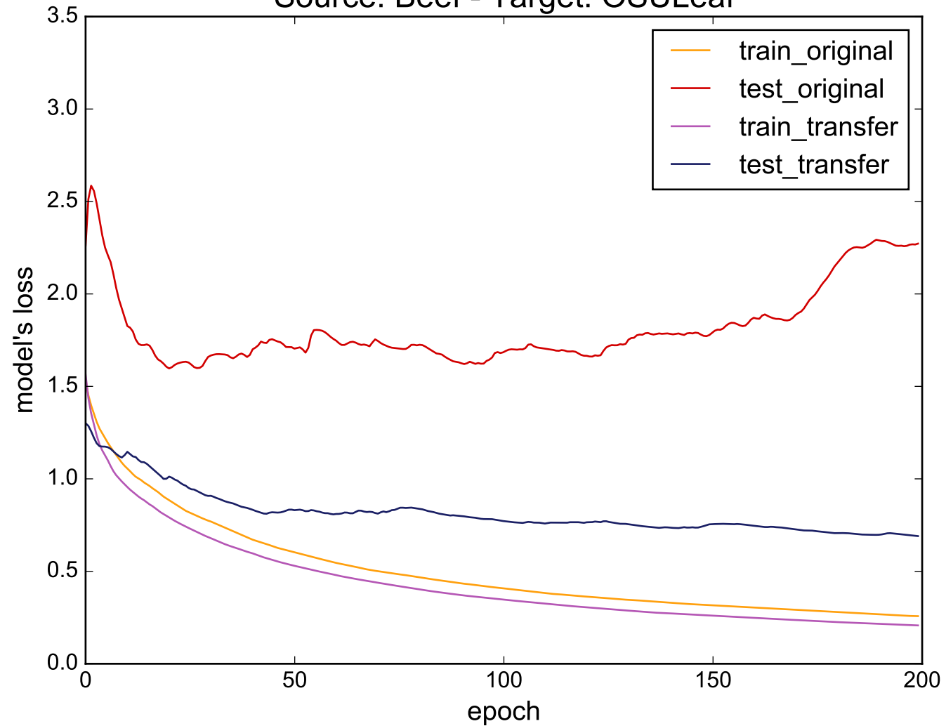
Source: Beef - Target: OSULeaf
