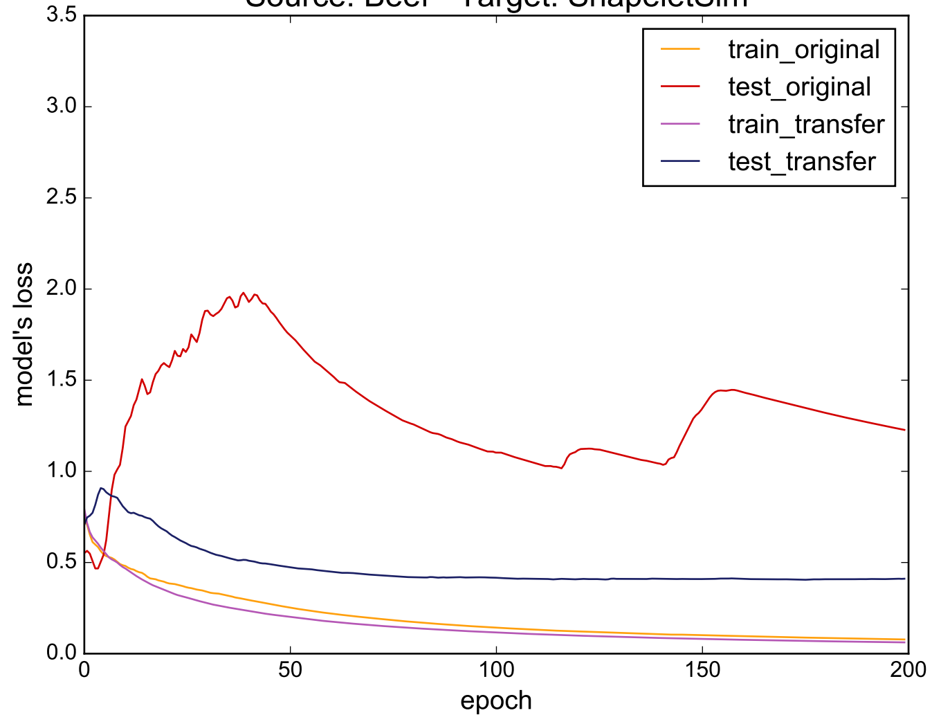
Source: Beef - Target: ShapeletSim
