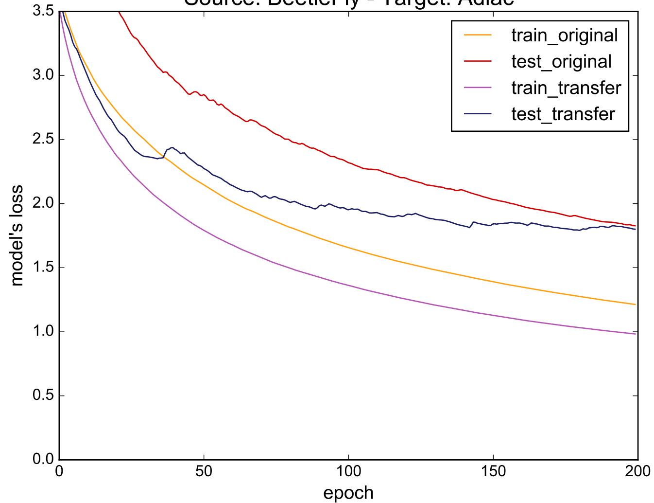
Source: BeetleFly - Target: Adiac
