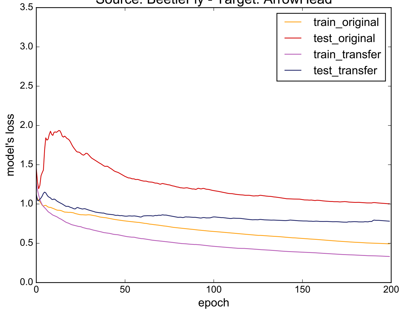
Source: BeetleFly - Target: ArrowHead
