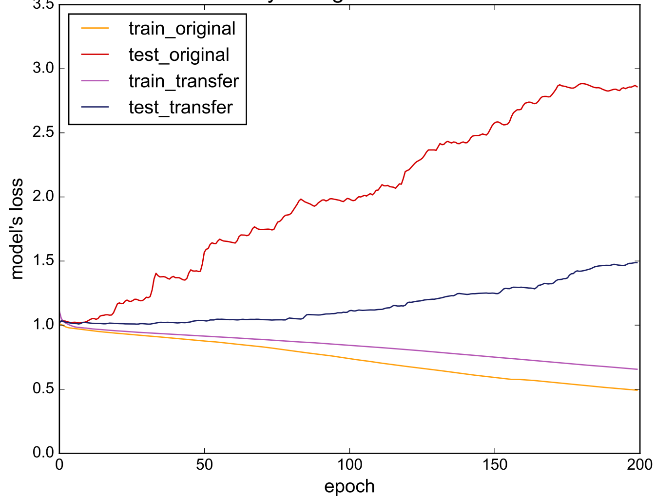
Source: BeetleFly - Target: ChlorineConcentration
