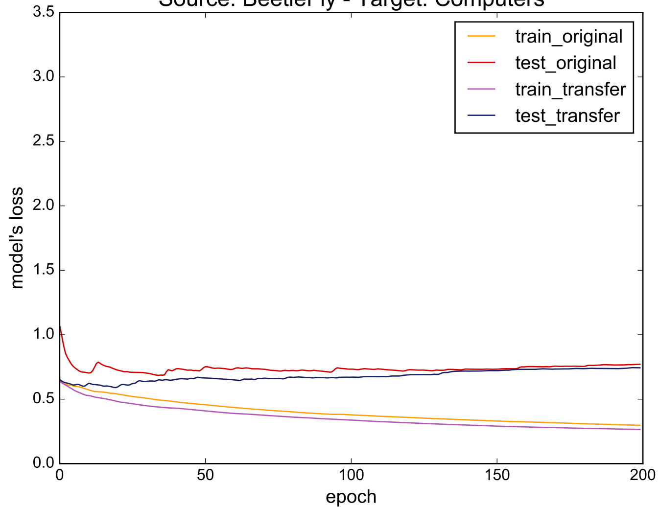
Source: BeetleFly - Target: Computers
