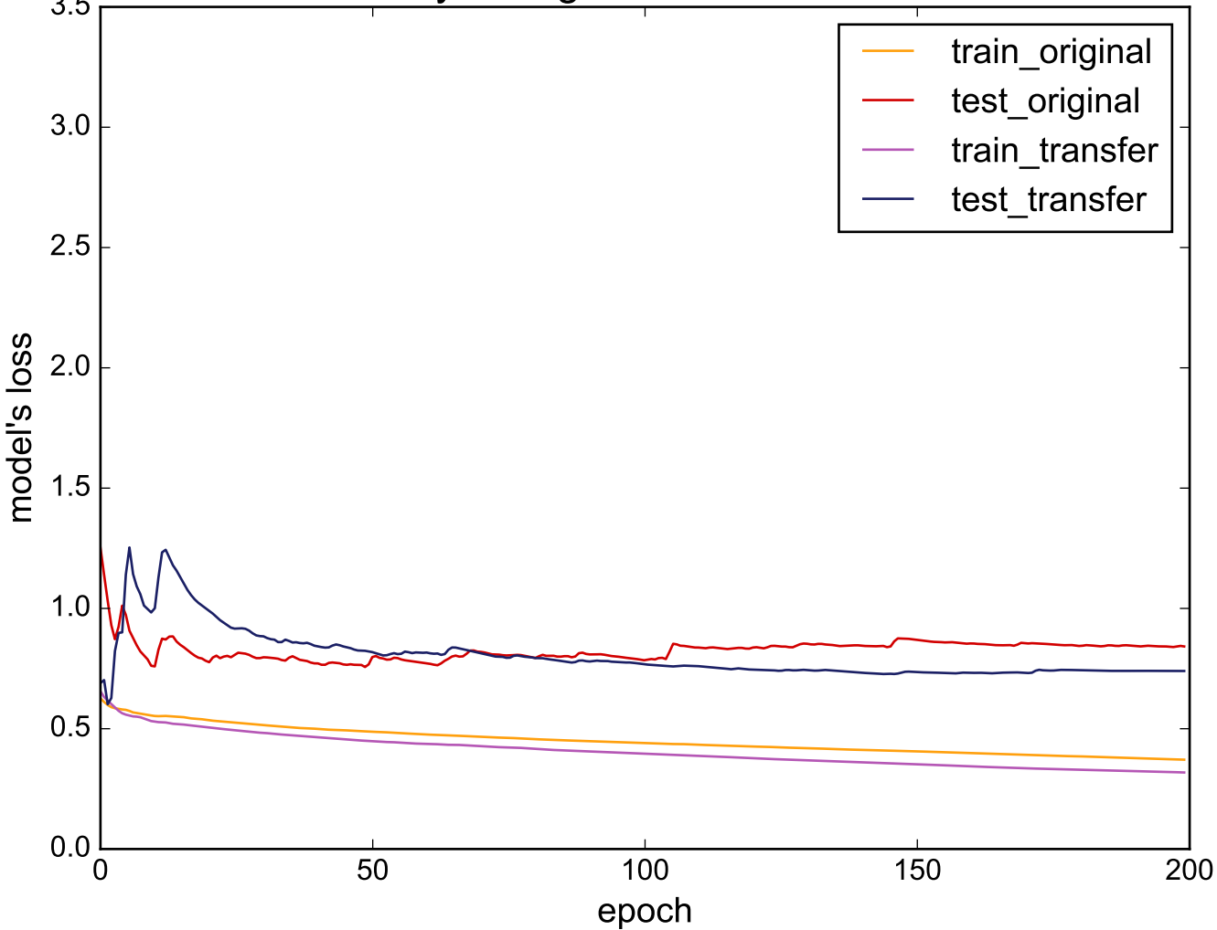
Source: BeetleFly - Target: DistalPhalanxOutlineCorrect
