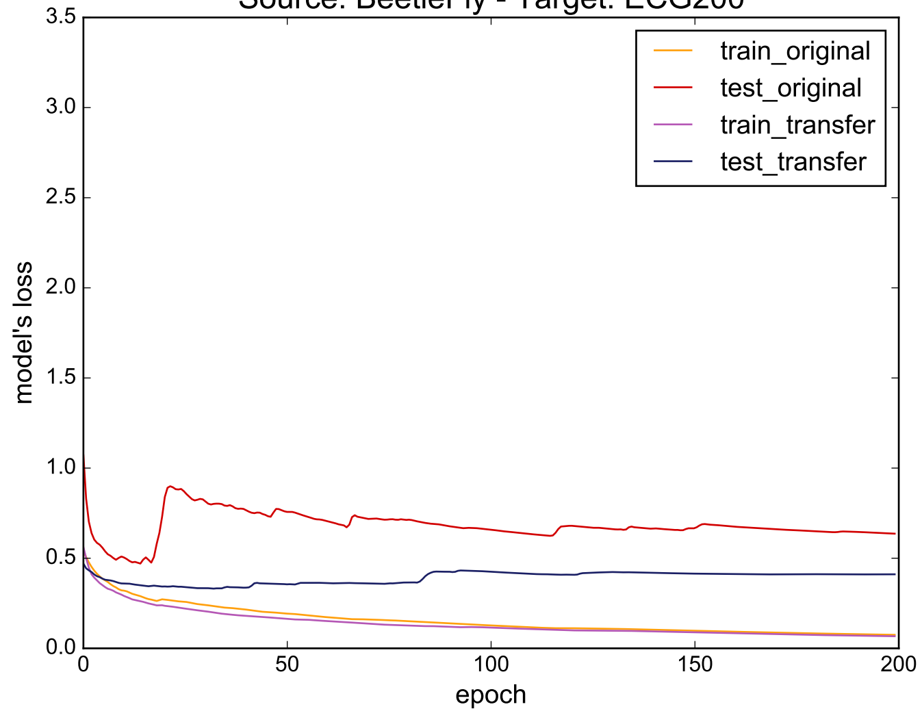
Source: BeetleFly - Target: ECG200
