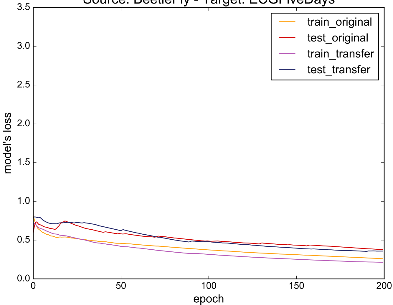
Source: BeetleFly - Target: ECGFiveDays
