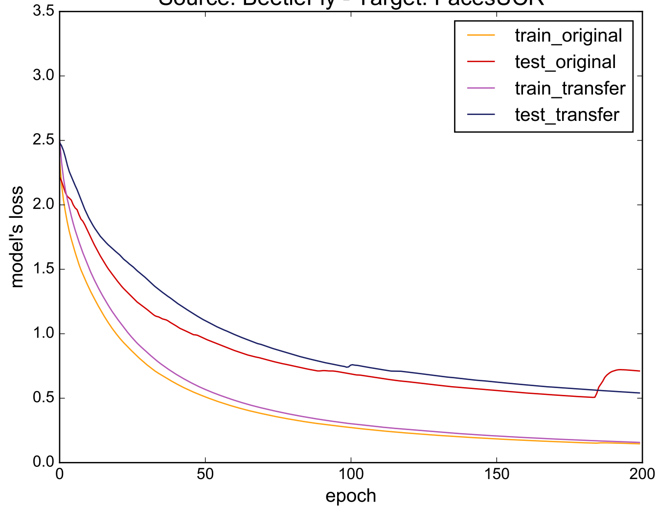
Source: BeetleFly - Target: FacesUCR
