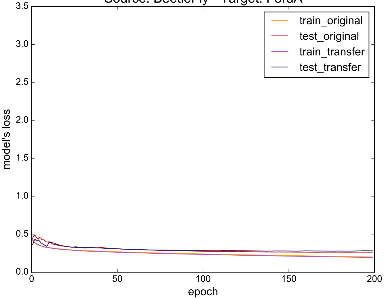
Source: BeetleFly - Target: FordA
