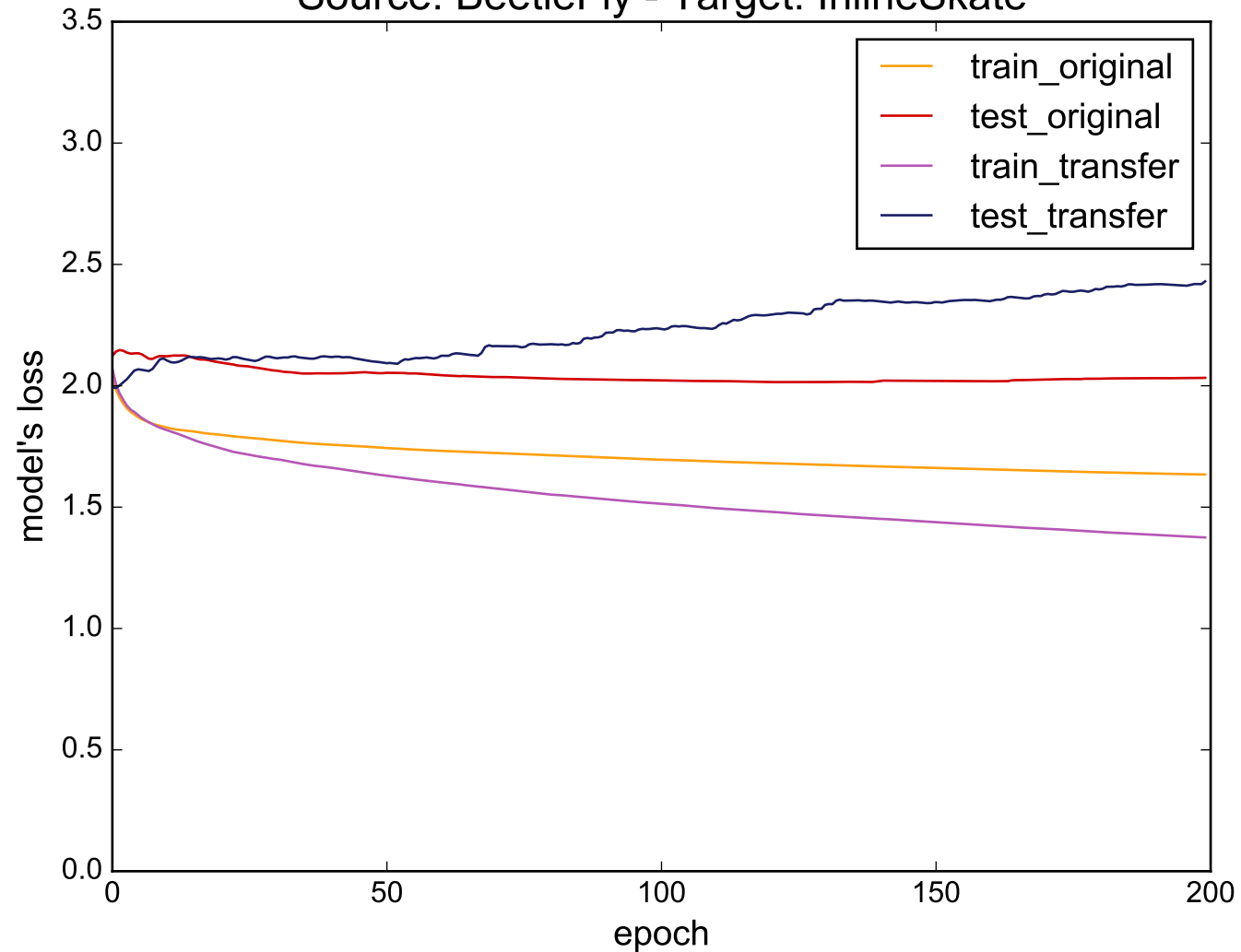
Source: BeetleFly - Target: InlineSkate
