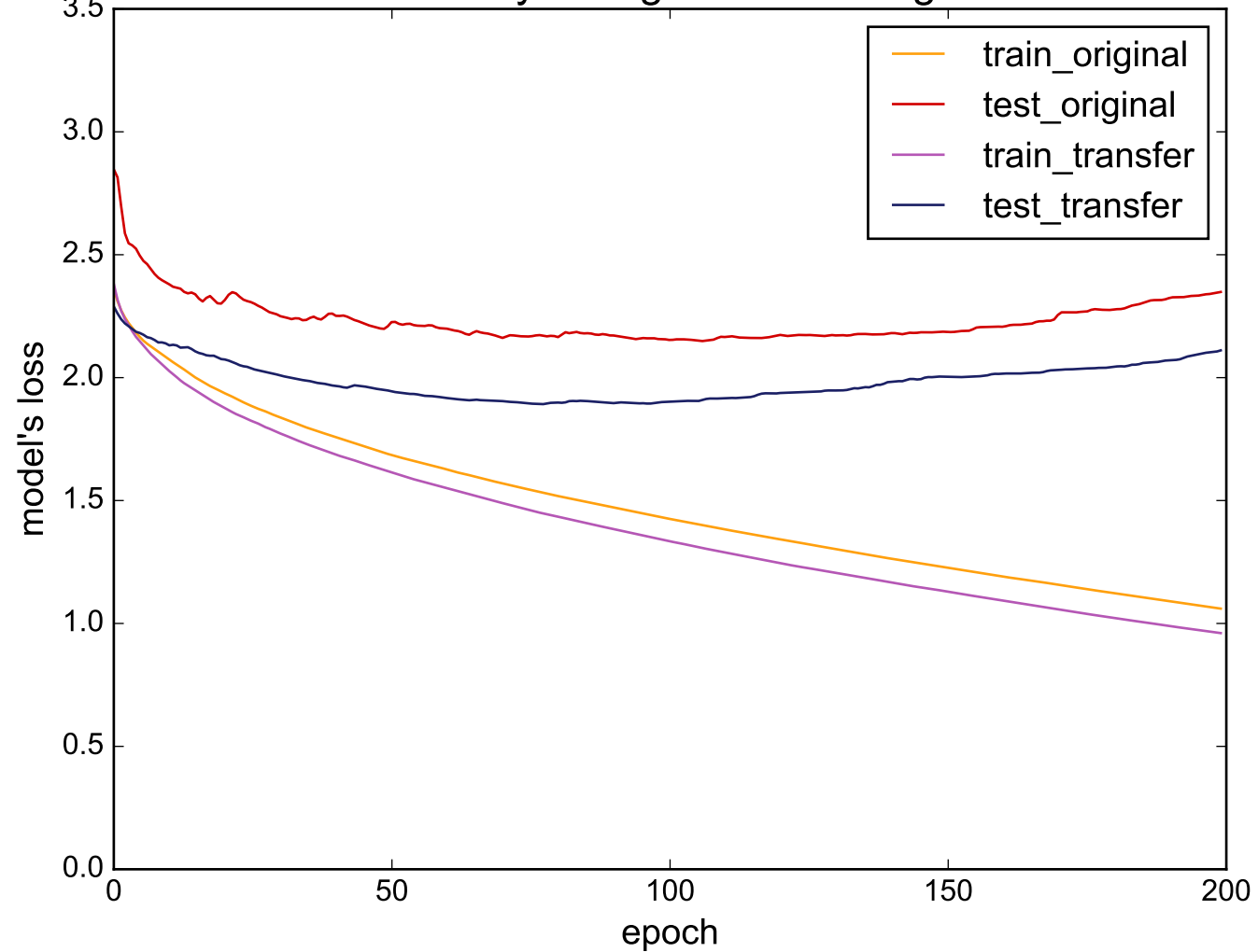
Source: BeetleFly - Target: InsectWingbeatSound
