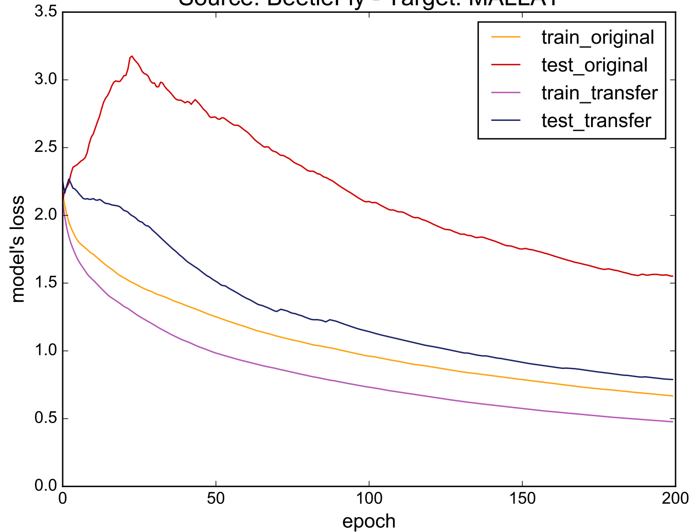
Source: BeetleFly - Target: MALLAT
