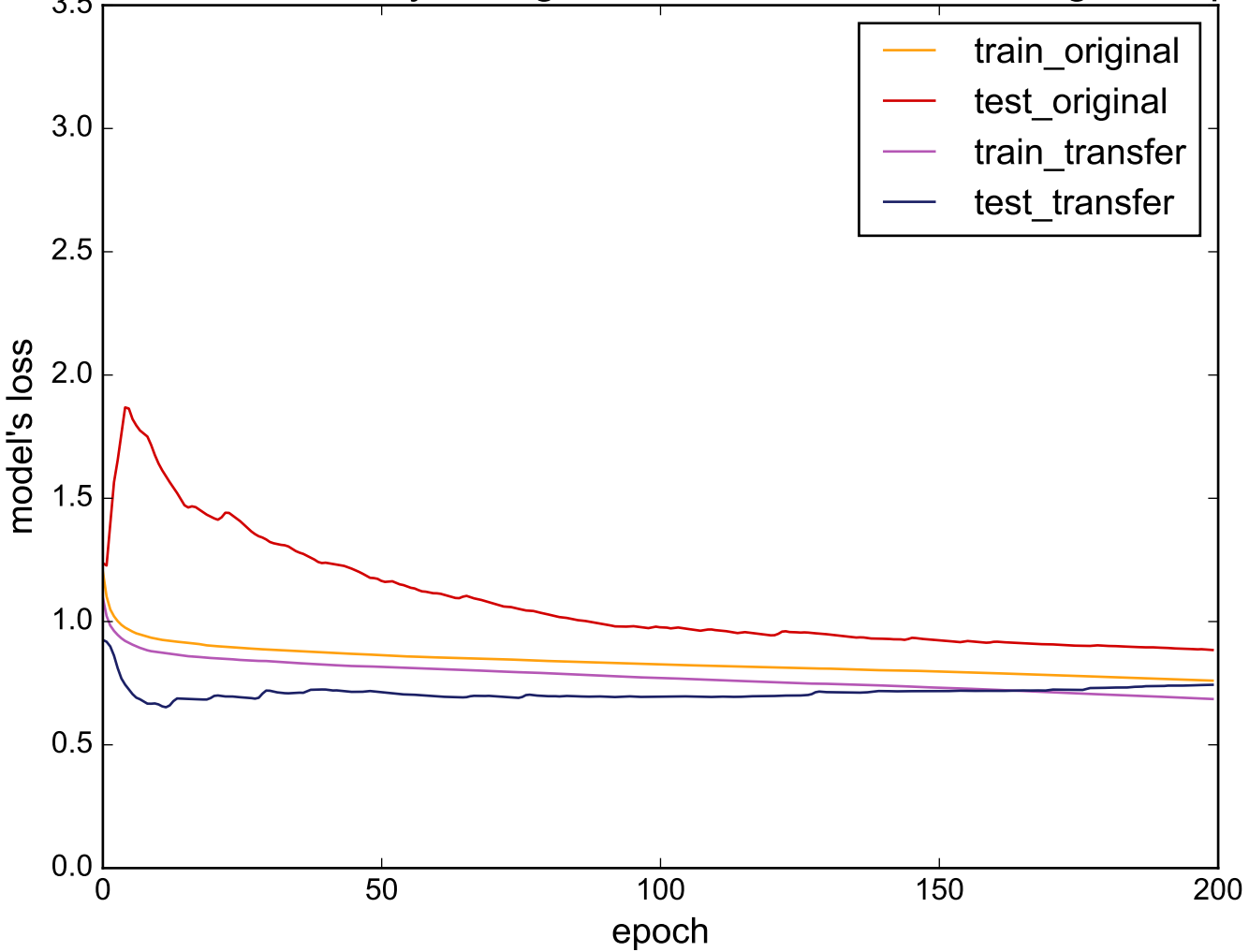
Source: BeetleFly - Target: MiddlePhalanxOutlineAgeGroup
