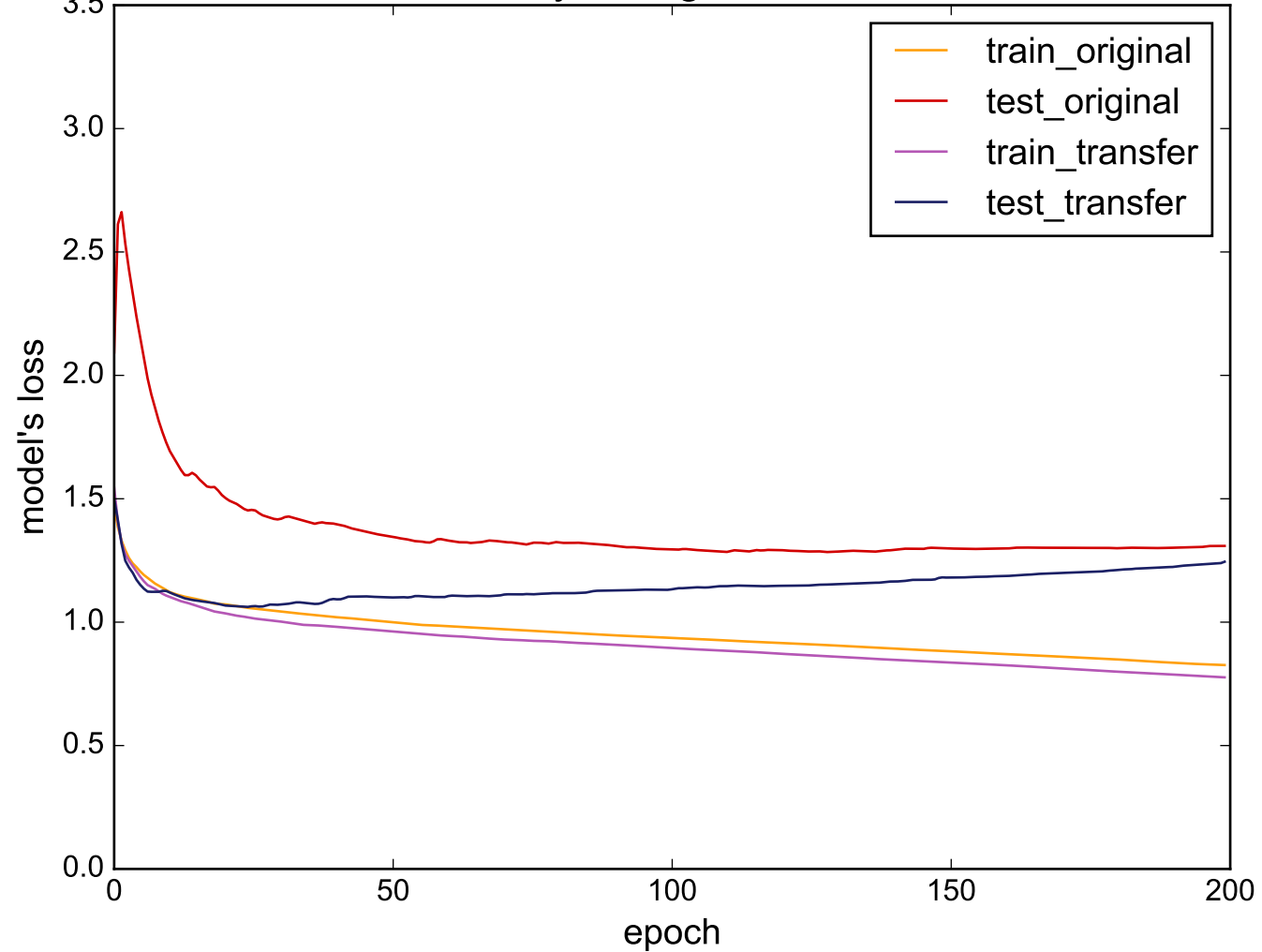
Source: BeetleFly - Target: MiddlePhalanxTW
