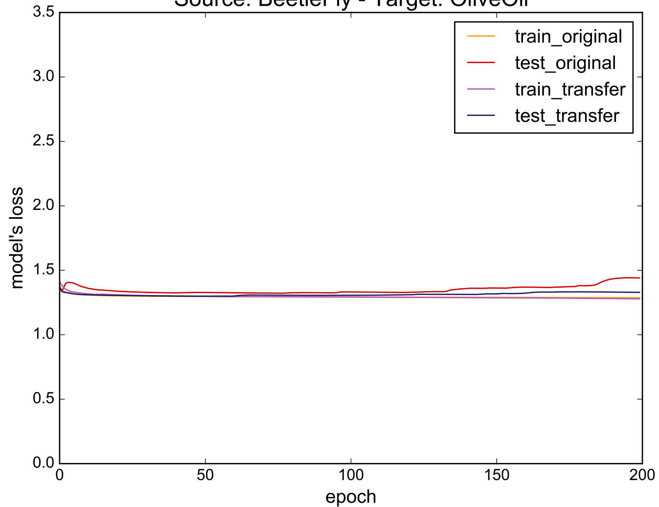
Source: BeetleFly - Target: OliveOil
