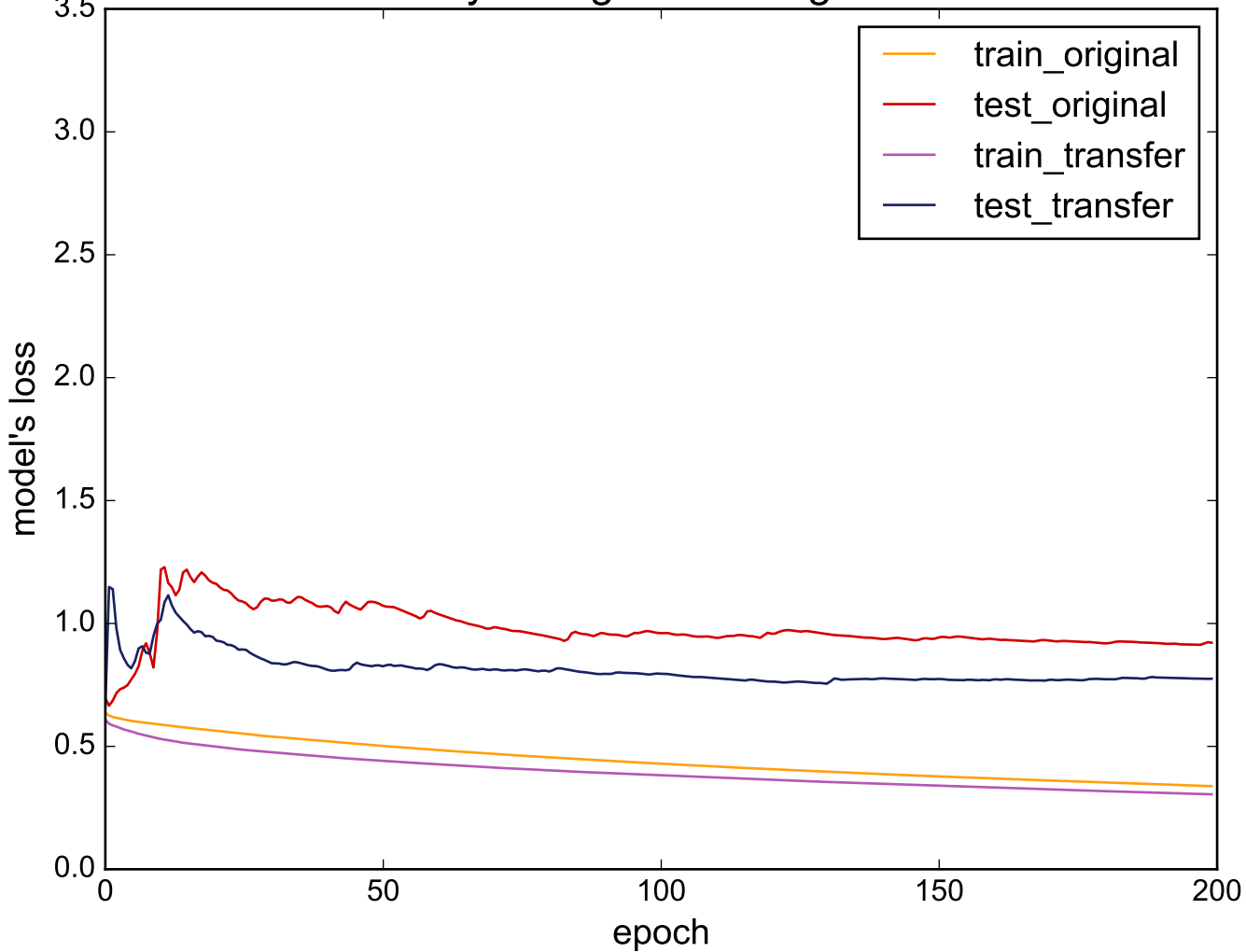
Source: BeetleFly - Target: PhalangesOutlinesCorrect
