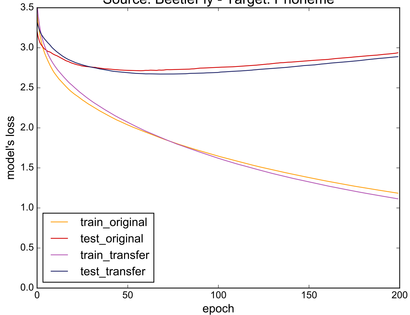
Source: BeetleFly - Target: Phoneme
