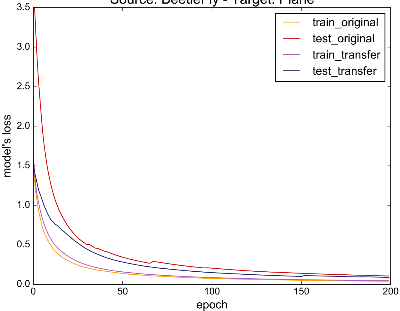
Source: BeetleFly - Target: Plane
