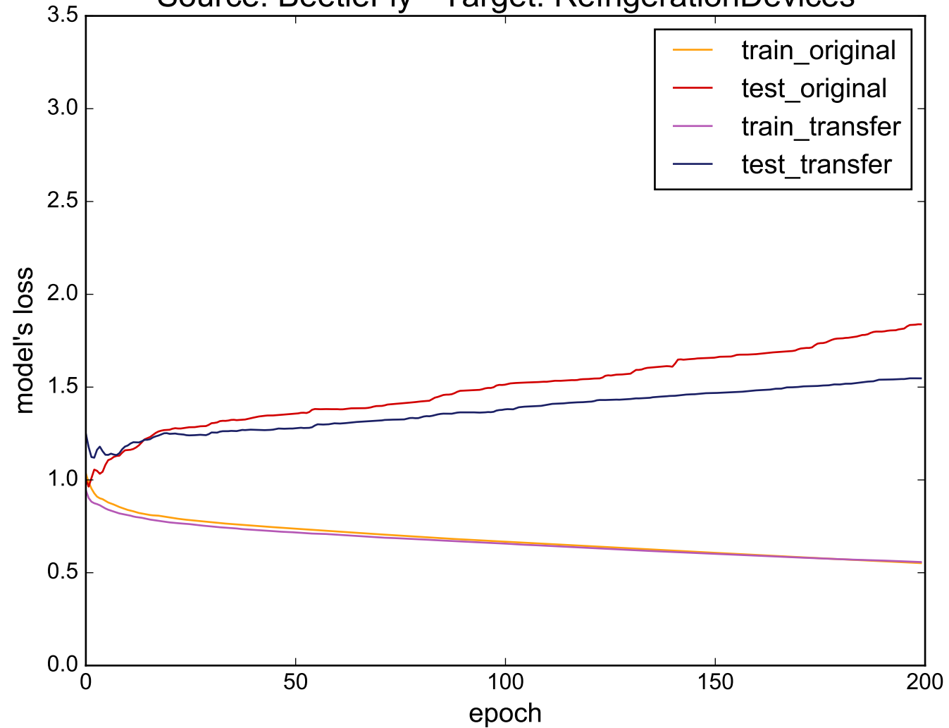
Source: BeetleFly - Target: RefrigerationDevices
