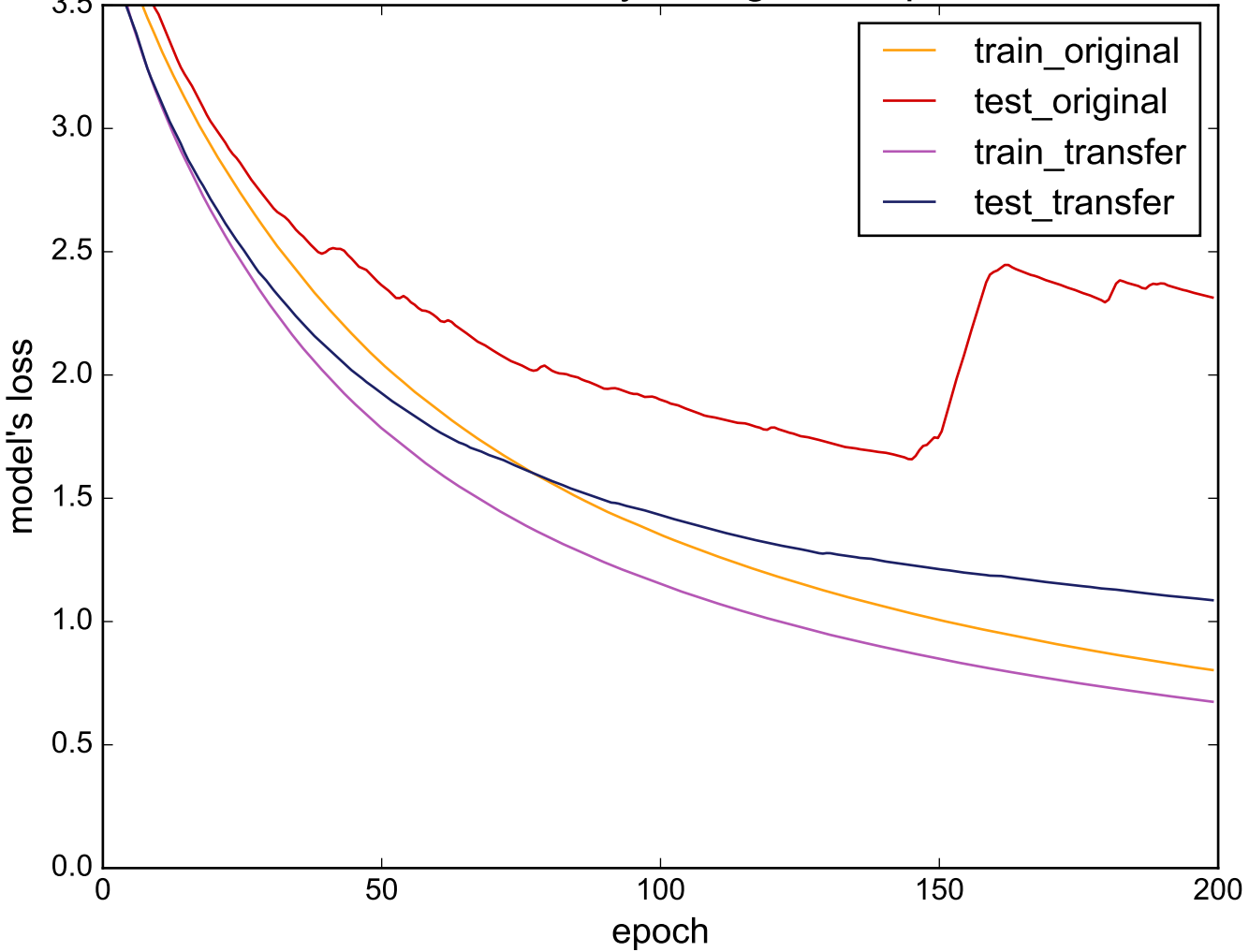
Source: BeetleFly - Target: ShapesAll
