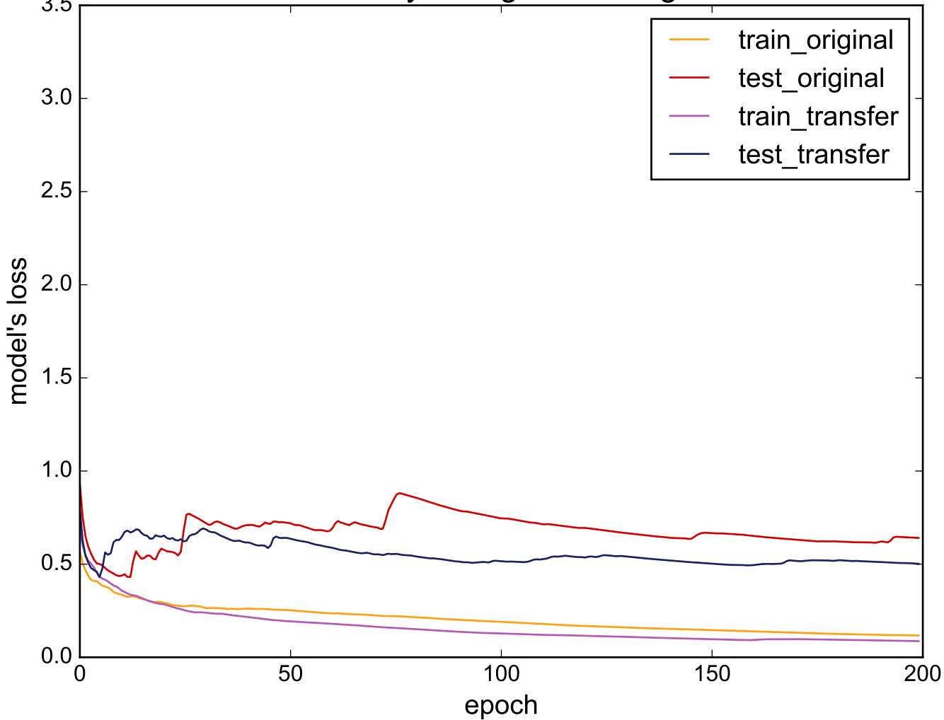
Source: BeetleFly - Target: ToeSegmentation2
