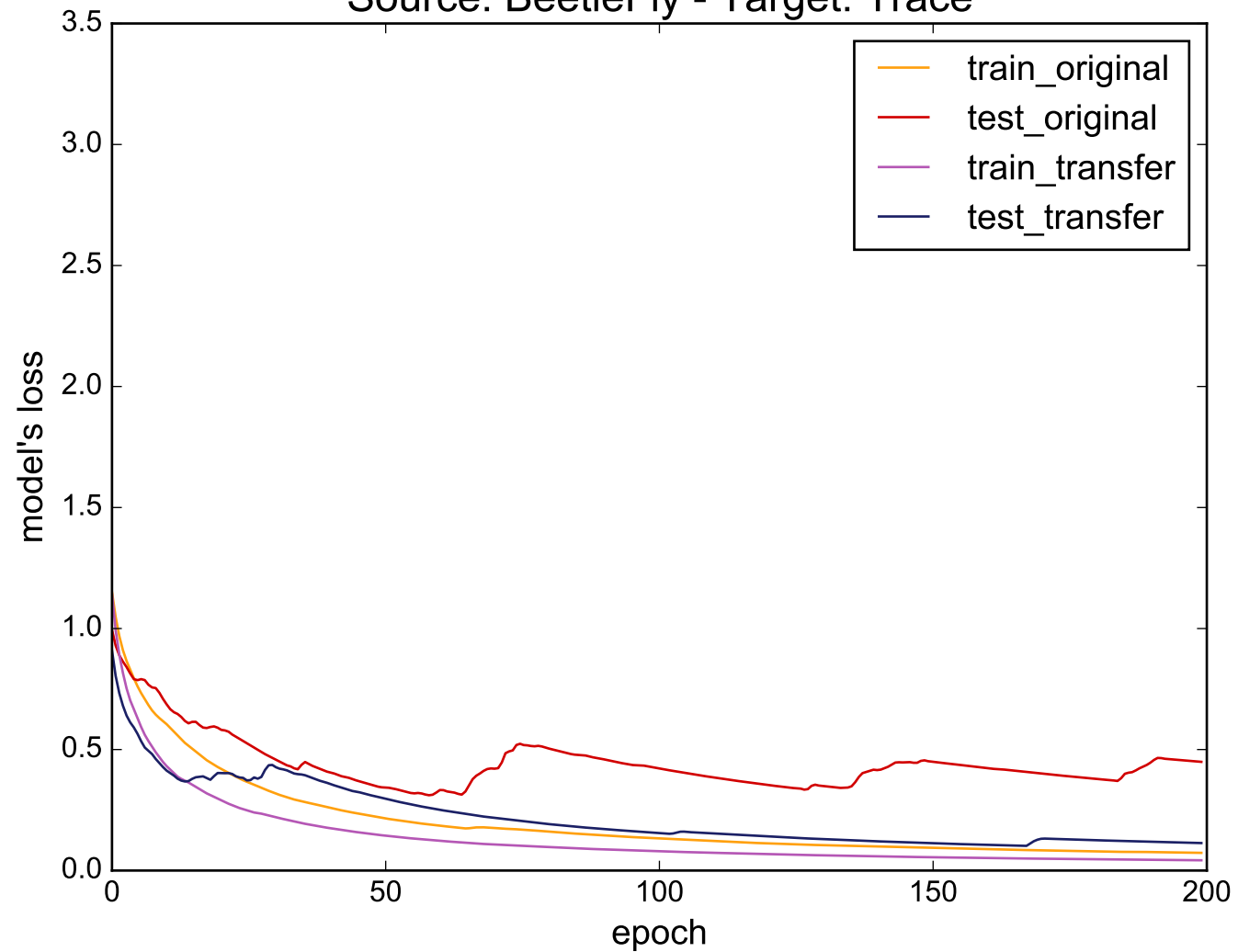
Source: BeetleFly - Target: Trace
