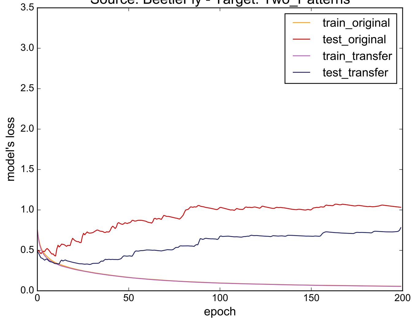
Source: BeetleFly - Target: Two_Patterns
