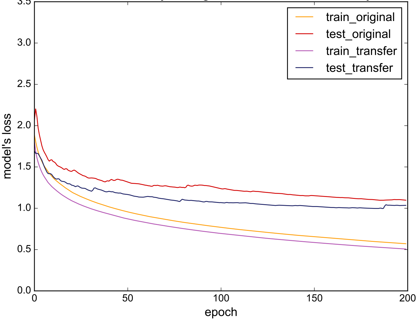
Source: BeetleFly - Target: UWaveGestureLibraryAll
