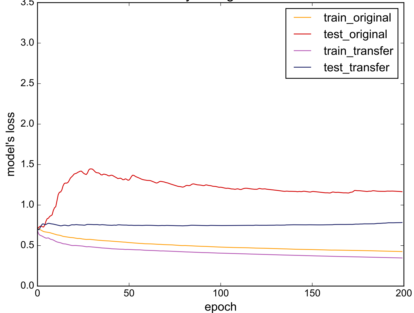
Source: BeetleFly - Target: WormsTwoClass
