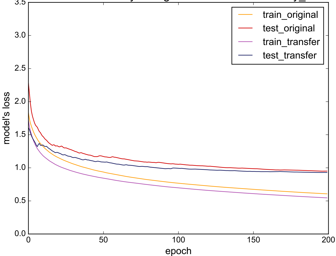
Source: BeetleFly - Target: uWaveGestureLibrary_X
