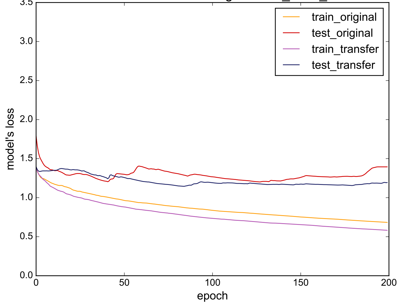
Source: BirdChicken - Target: CinC_ECG_torso
