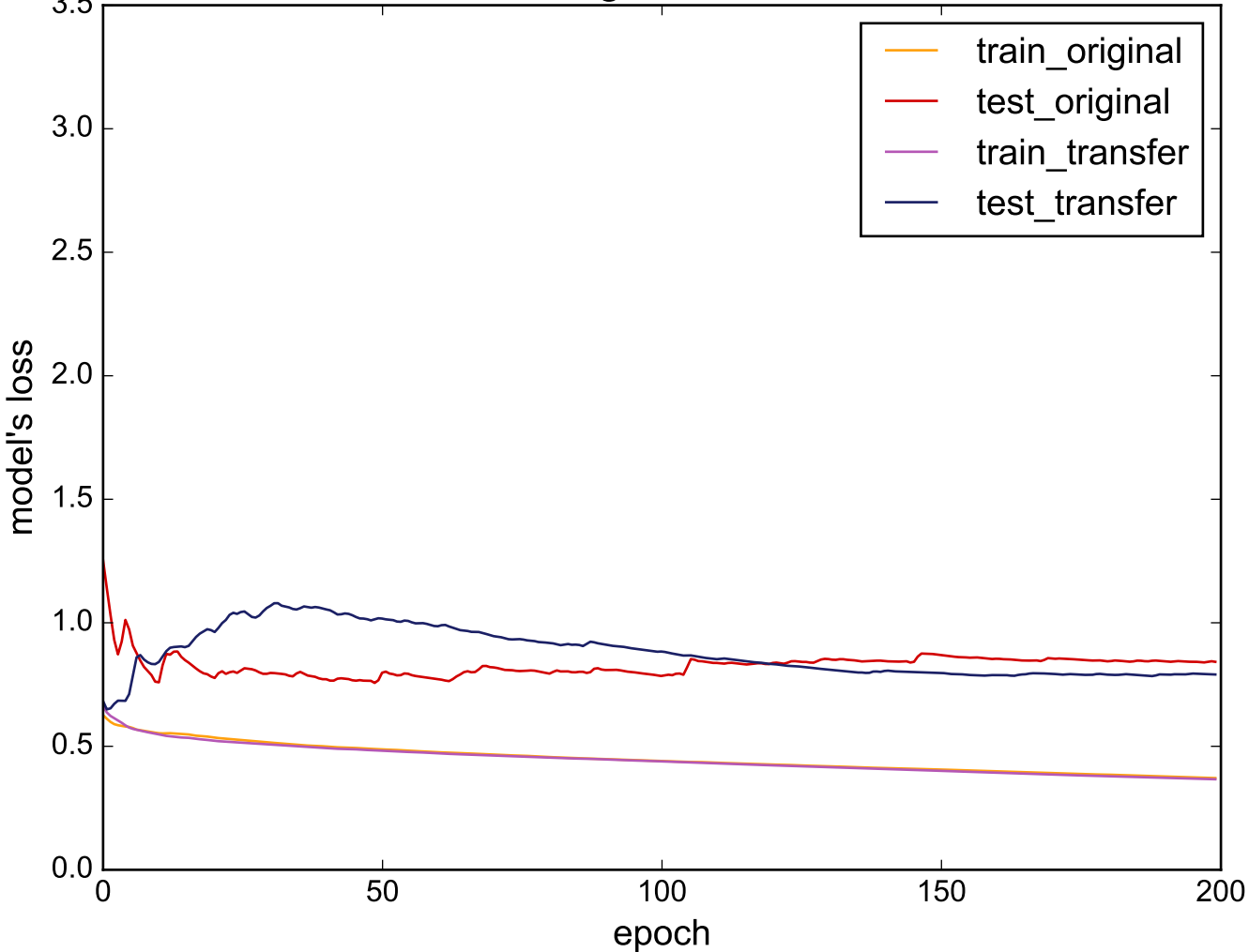
Source: BirdChicken - Target: DistalPhalanxOutlineCorrect
