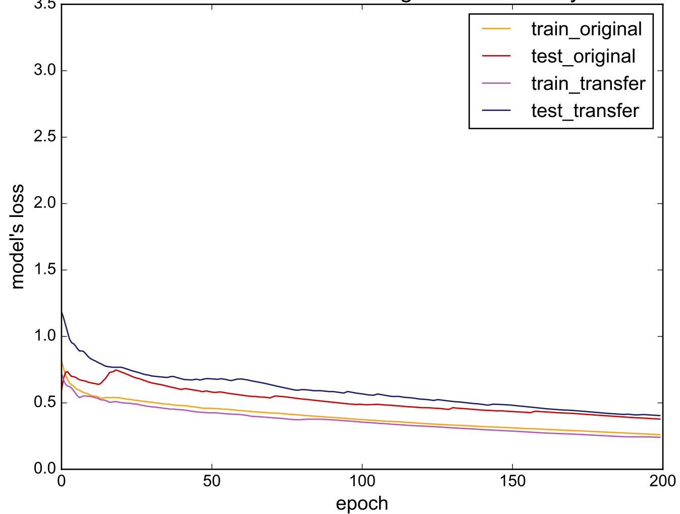
Source: BirdChicken - Target: ECGFiveDays
